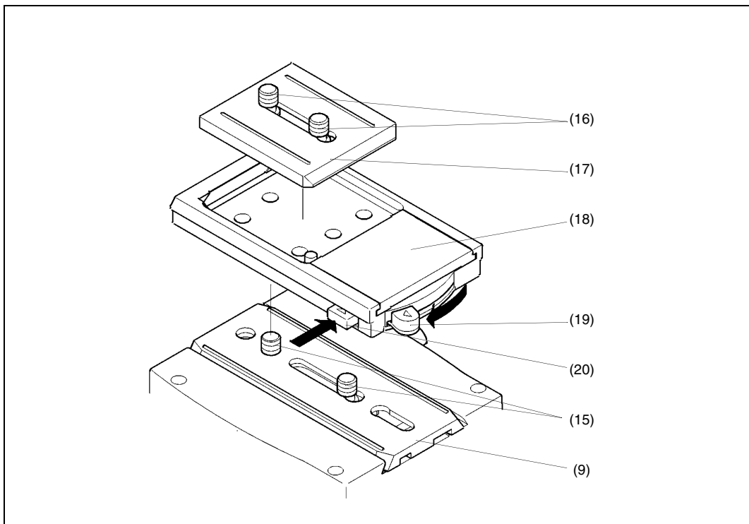
Mounting the camera (optional Quickfit adaptor)
