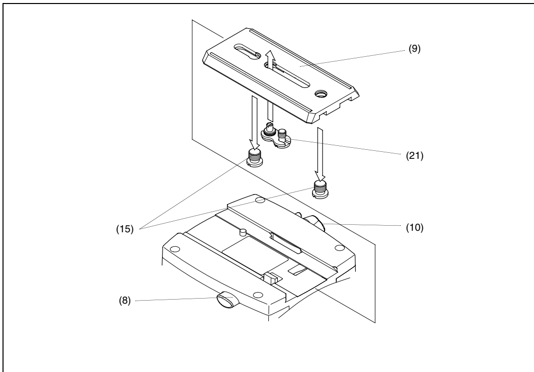
Mounting the camera (VHS adaptor)
